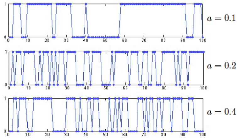
Figure 2: Simulations of the two-state Markov chain
